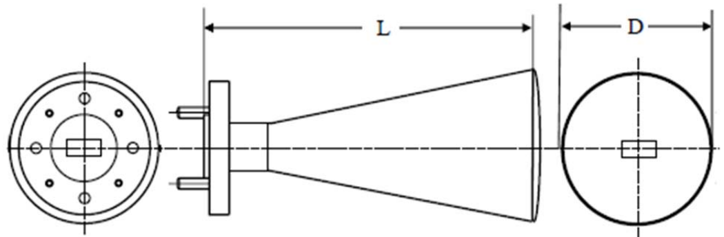
Outline Drawing Standard Gain Antenna
