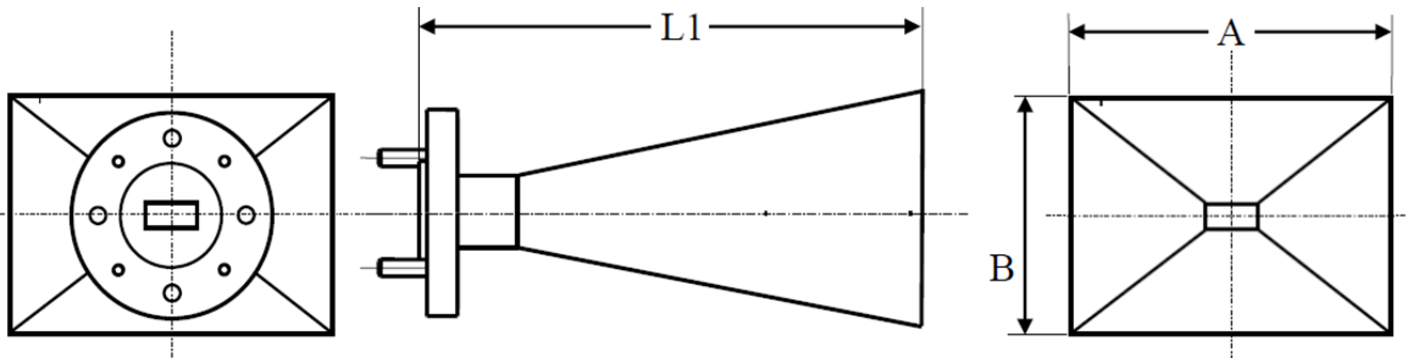
Outline Drawing Gain Pyramid Horn Antenna
